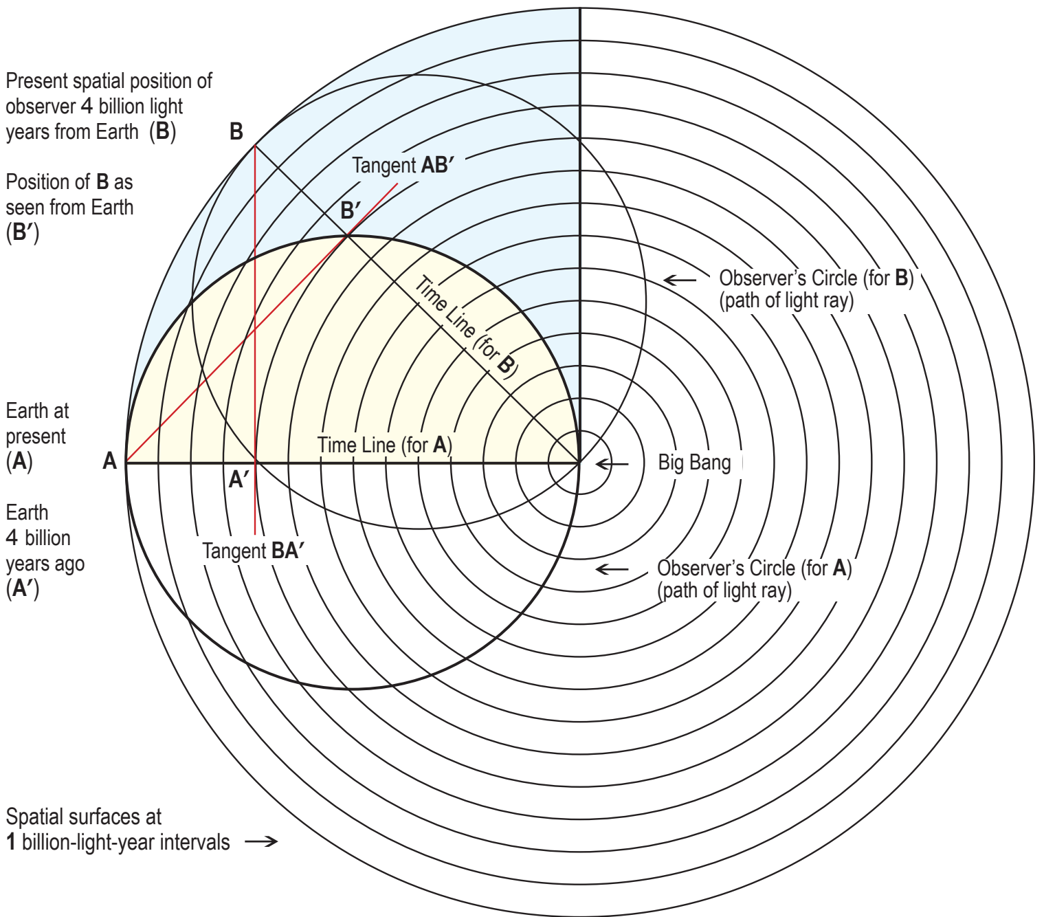
Figure 1: The Spacetime Map Diagram
